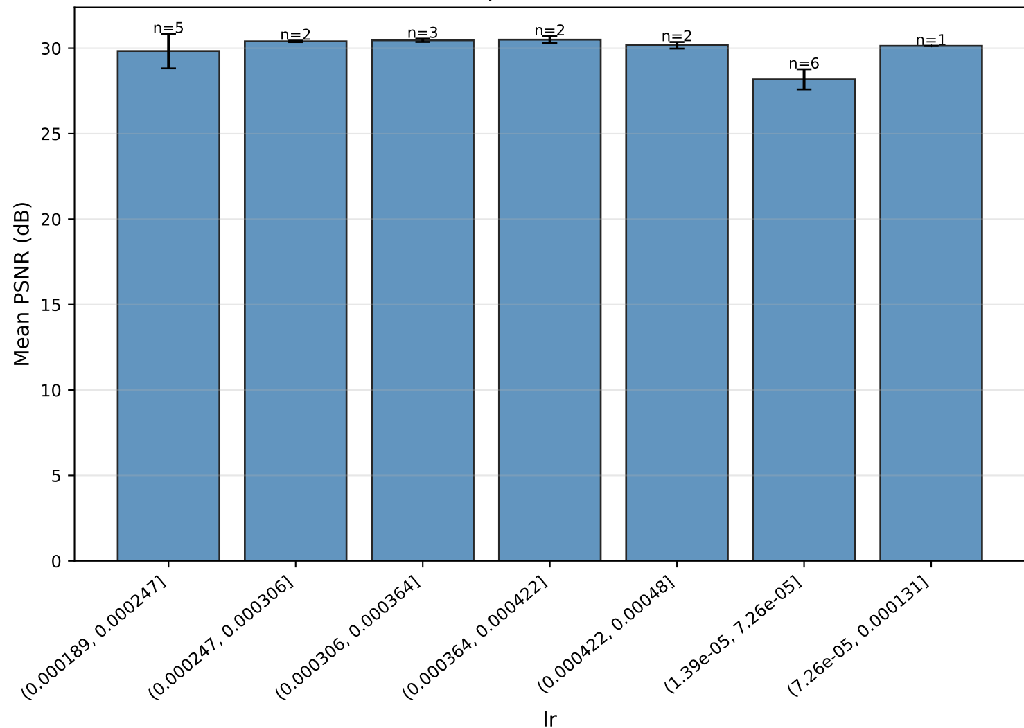
Mean PSNR per value of l_r — ELAN
